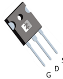
TO-247-3
